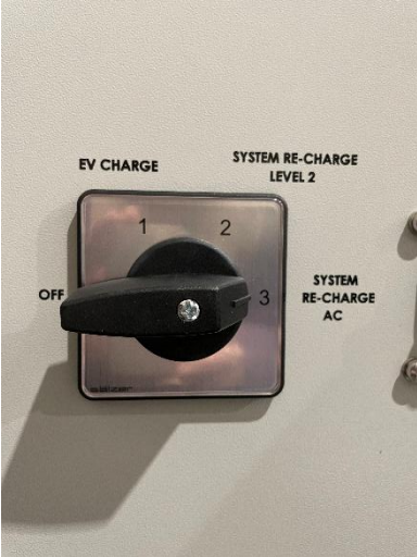
Figure 15—Selector Switch in SYSTEM RE-CHARGE AC (3) position
