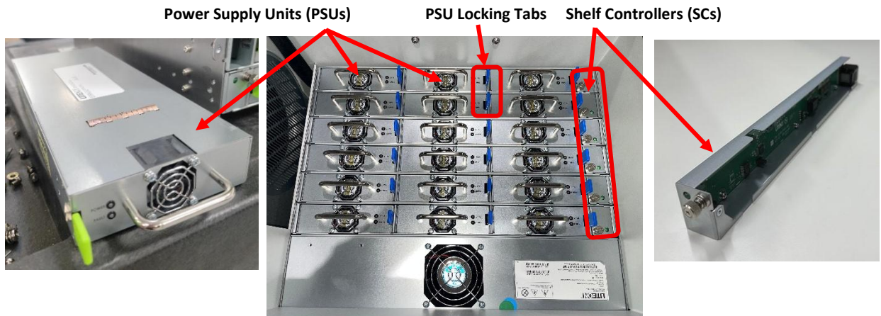
Figure 8—Orientation to Power Supply Units (PSUs) and Shelf Controllers (SCs) when loaded in power
