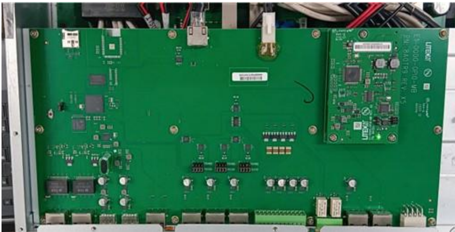
Figure 15 – MCU Shelf/Board Unit
