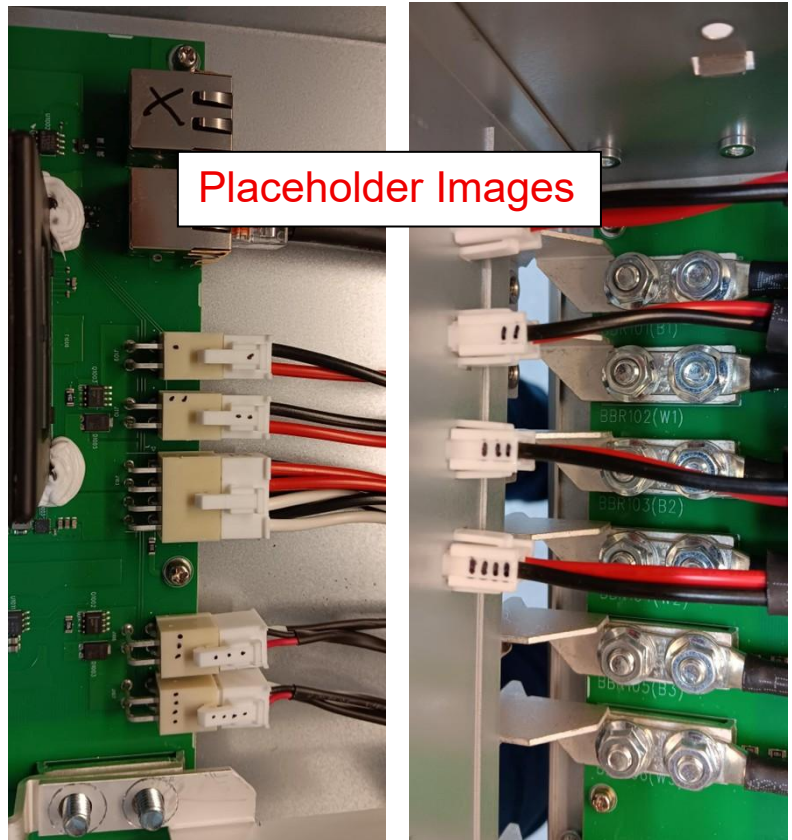
Figure 17 – Smaller PCB installed in bottom of Rack Controller
