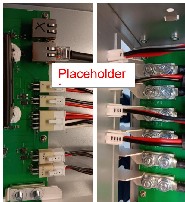
Figure 1: Bias Supply, smaller of two PCBs installed at bottom of Rack Controller in this 60 kW Bi-Directional Charger
