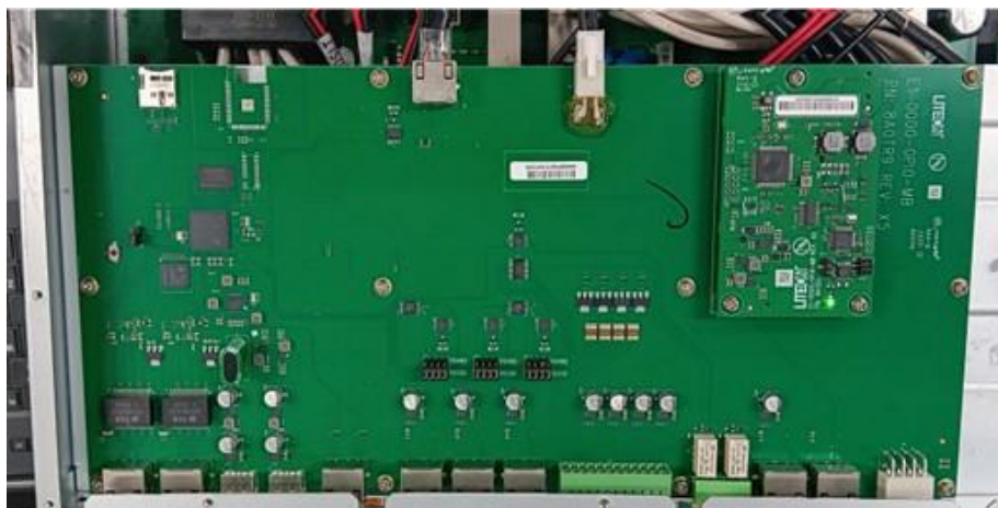
Figure 1: MCU Board installed in this 60 kW Bi-Directional Charger includes one larger and one smaller PCB
