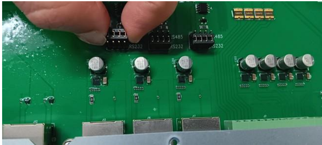
Figure 17 – Transfer new MCU board by hand, only 4 lower pins exposed
