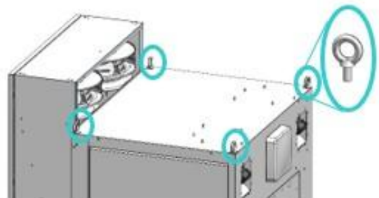
Figure 18 – Installing eye bolts
