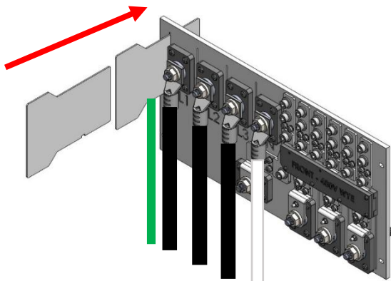
Figure 47 - AC Input Wiring for different AC Input Power Configurations
