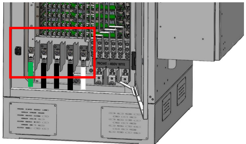
Figure 47 - AC Input Wiring for different AC Input Power Configurations
