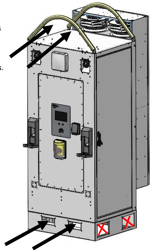
Figure 15 – Forklift forks may be inserted into either the two open front panels or 2 lifting straps connected to eye bolts on top of charger
