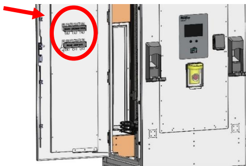
Figure 43 - Inside left door is shipping/storage location of 2 configuration bus bars
