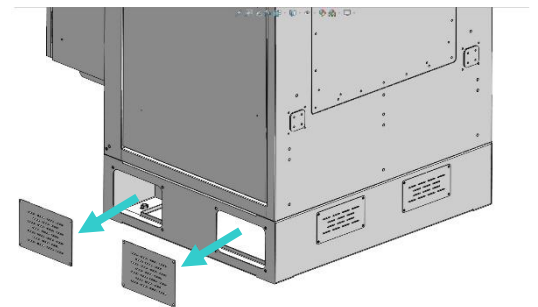
Figure 13 - Removing left and right access panels to access 4 hex bolts and washers securing charger to pallet
