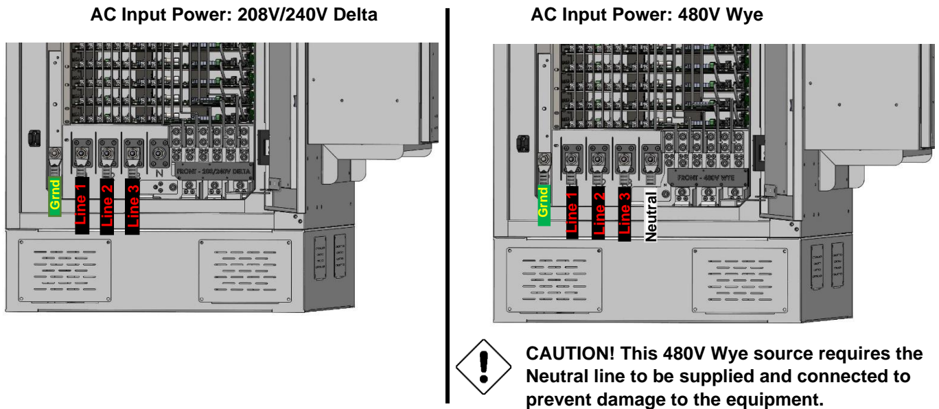
Figure 45 - AC Input Wiring for different AC Input Power Configurations
