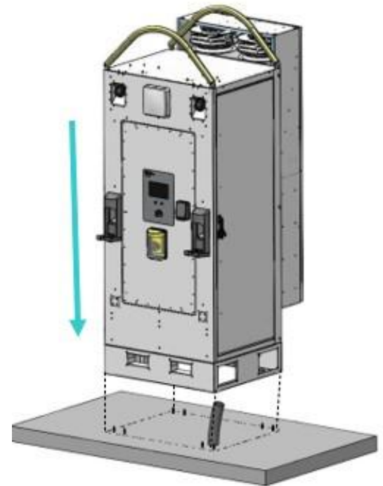
Figure 19 - Lower Fast Charger onto eight pre-installed wedge anchors
