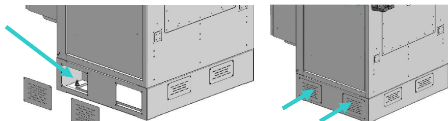
Figure 20 – Tighten washer-nut sets over wedge anchors and then re-attach all lower panel
