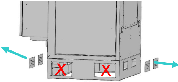
Figure 14 - Removing front and back access panels to prepare for forklift to lift off pallet
