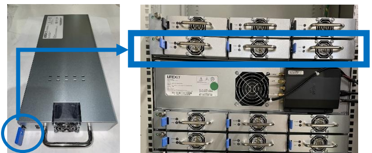
Figure 33 – Rectifier modules (blue tabs) installed in lower shelf of Inverter Shelf Set
