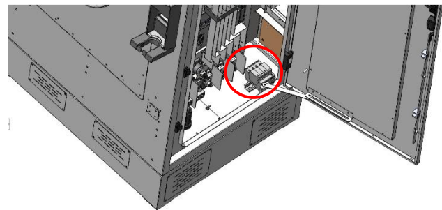
Figure 54 - Surge Protective Device that contains replaceable surge modules
