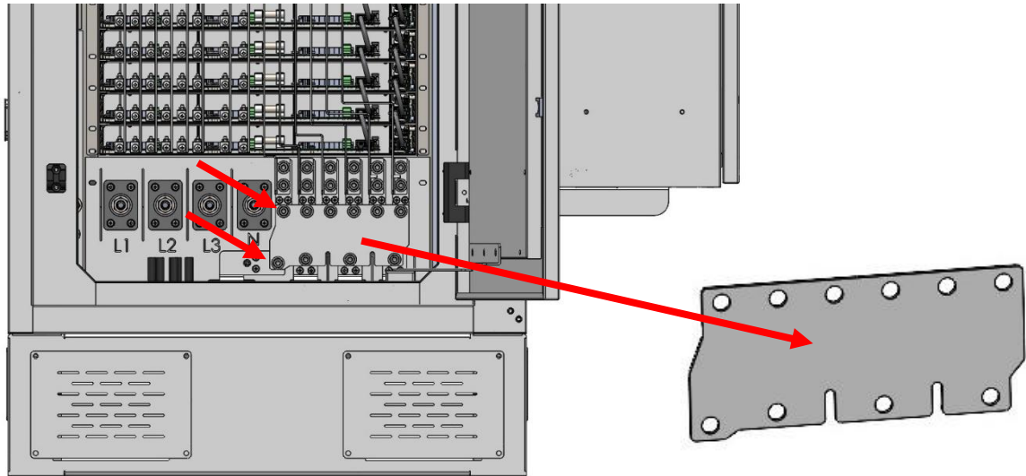
Figure 41 - M6 and M8 socket head cap screws must be removed to remove plastic spacer plate
