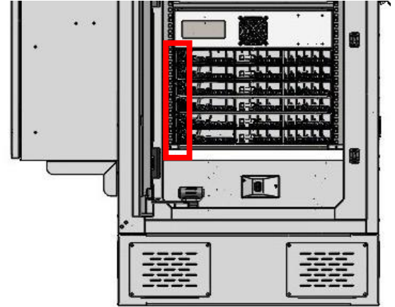
Figure 26 – Empty shelves in charger's bottom power stack with six empty shelf controller slots highlighted
