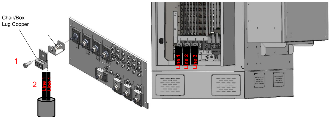
Figure 46 - (1) Chair/Box Lugs (not provided) with Copper Extensions (provided) can be used in place of Ring Terminals (2) when wiring AC input Lines 1, 2, or 3
