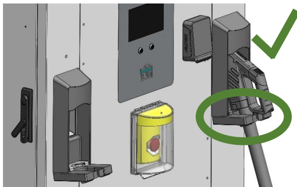
Figure 51 - Charging Cable handle docked correctly with cable behind holster's rubber gate
