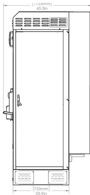
Figure 4.3 - Right Side, Depth of 120kW Charger
