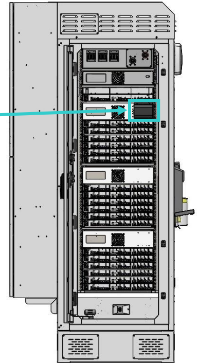
Figure 35 - Locating pre-installed cellular modem inside left-side door
