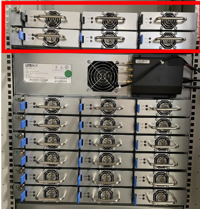
Figure 31– Inverter Shelf Set has two dedicated shelves: Upper Shelf for three (3) Inverter modules (with black tabs) Lower Shelf for three (3) Rectifier modules (with blue tabs)
