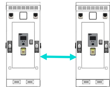
Figure 6 – Minimum space between chargers is 42 inches (1067 mm)
