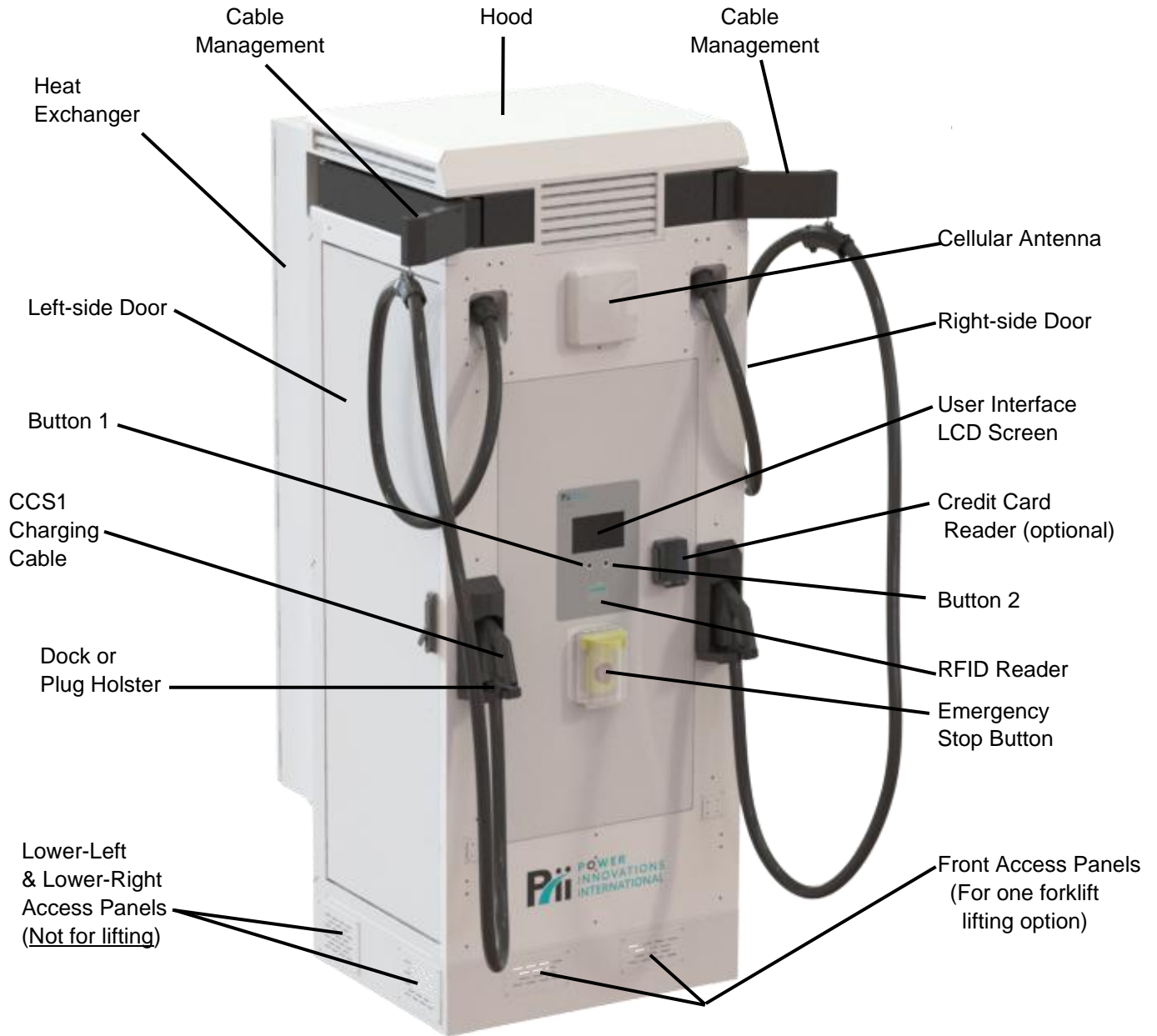
Figure 2 - EV Fast Charger Model EVFC180-26BS – with Dual 6 m Charging Cables (with Cable Management), RFID Reader and Card Reader
