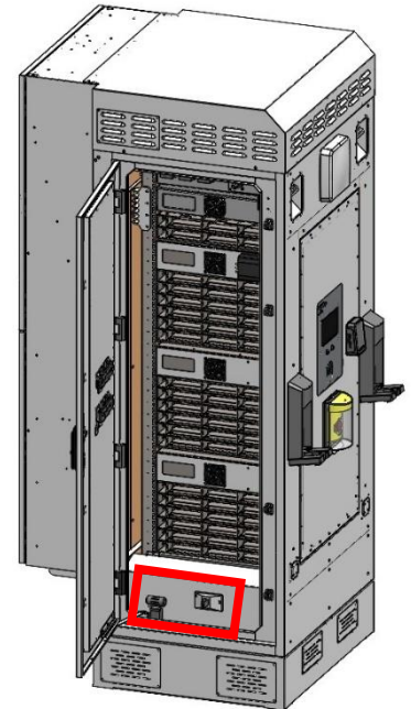
Figure 21 – Main Switch and removable handle in a 180 kW EV Fast Charger (inside left-side door)
