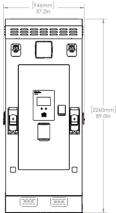
Figure 4.1 - Front View with Height and Width of 120kW Charger
