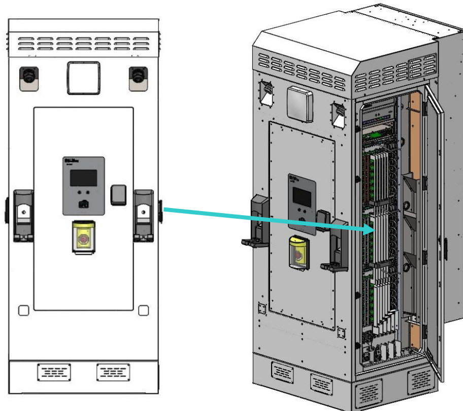
Figure 37 - Opening EV Fast Charger's right-side door
