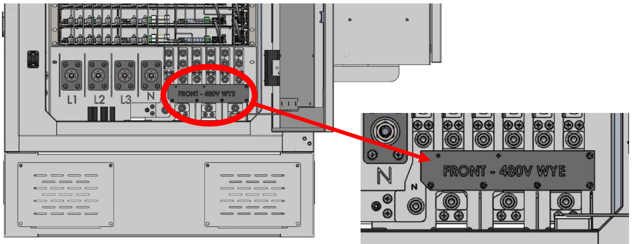
Figure 44 - FRONT – 480V WYE Configuration shown secured on Bus Bar
