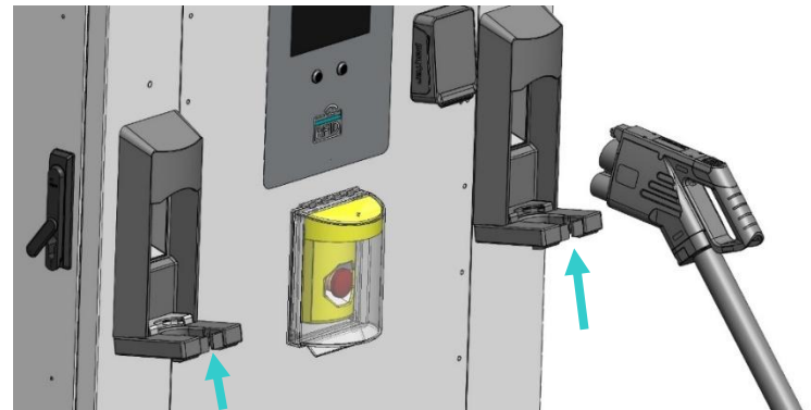
Figure 50 - Charging Cable holsters have a rubber gate that helps ensure properly seated handle
