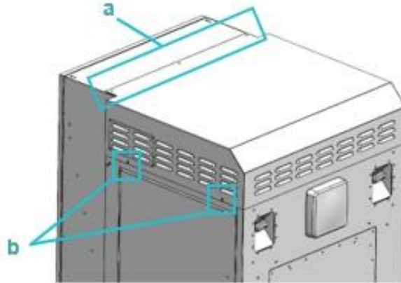
Figure 16 - Three screws and rubber washers on top of hood and four screws on upper-left and upper-right of hood secure hood to charger
