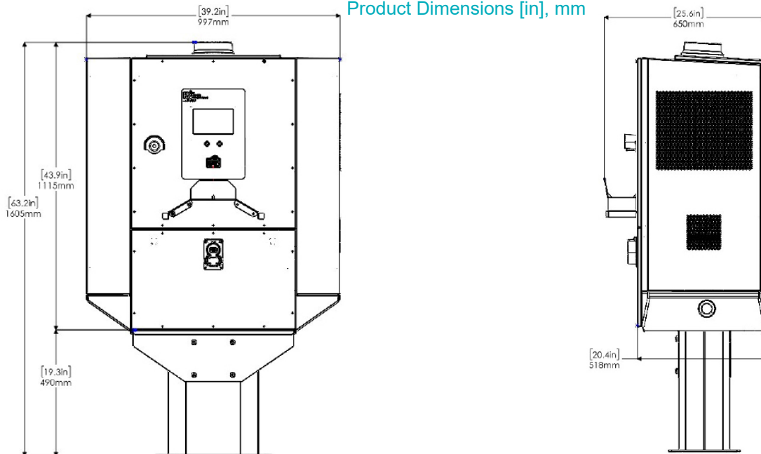
Product Dimensions [in], mm
